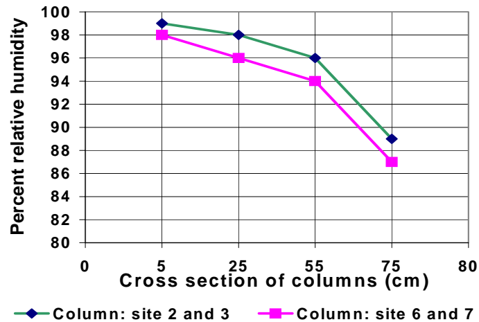
Fig. 6: Humidity profiles through 2 columns of Elgeseter Bridge starting from western faces.
