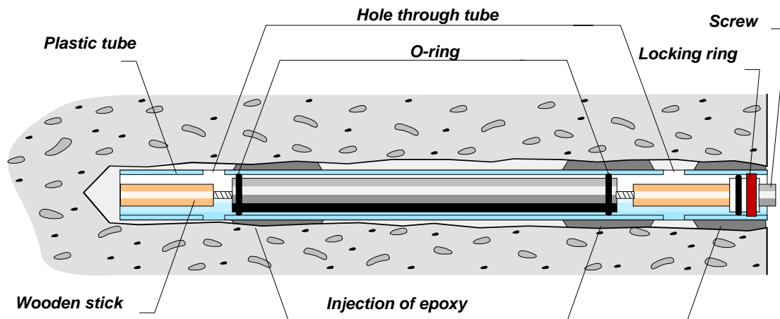
Fig. 3: Plastic tube mounted with 2 wooden sticks. Note that the contact between concrete and plastic tube has been injected with epoxy sealers. Diameter of the tube is 20 mm.
