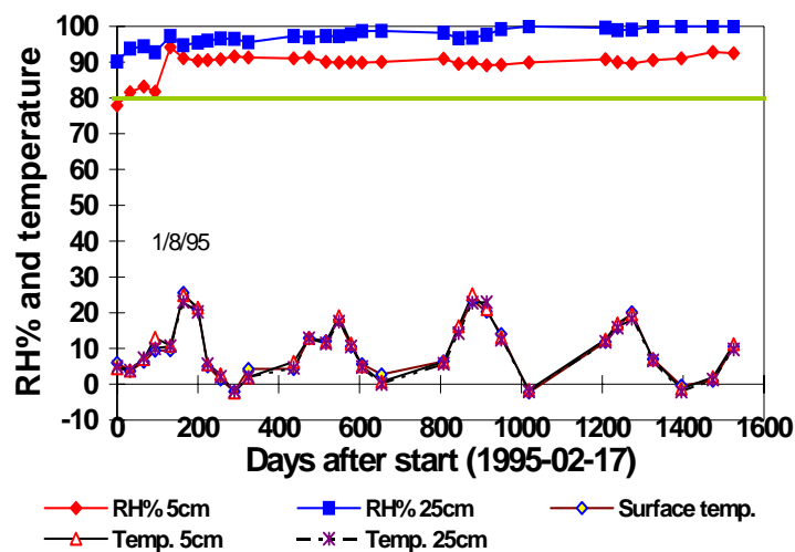
Fig. 5: Relative humidity and temperature (°C) during 4 years.
