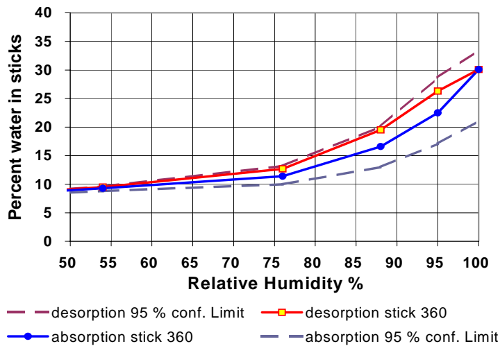
Fig. 1: Calibration curves for wooden stick no.360. In the figure the 95% confidence limits from 112 wooden stick is shown with broken line
