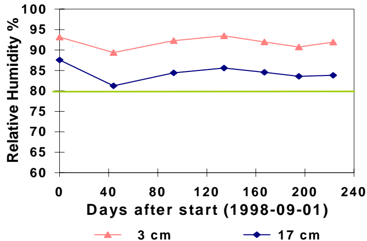
Fig. 7: Relative humidity measured 3 cm and 17 cm from outer surface in location no. 9.
