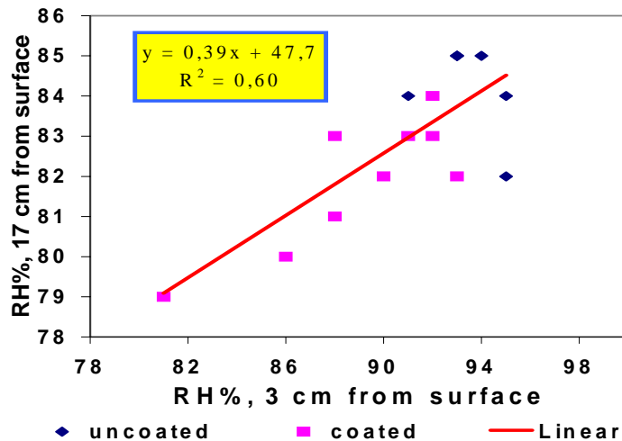
Fig. 8: Correlation of humidity measurements 3-cm respectively 17-cm from outer surface
