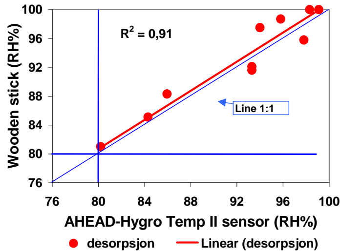
Fig. 2: Correlation between wooden stick with use of the desorption curve and AHEAD hygrotemp II sensors.
